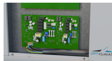
Power Connection Board
