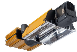
Dimlux Expert HPS Fixture
